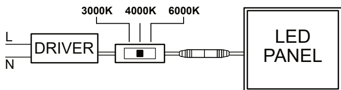
CCT switch for Premium LED panels
